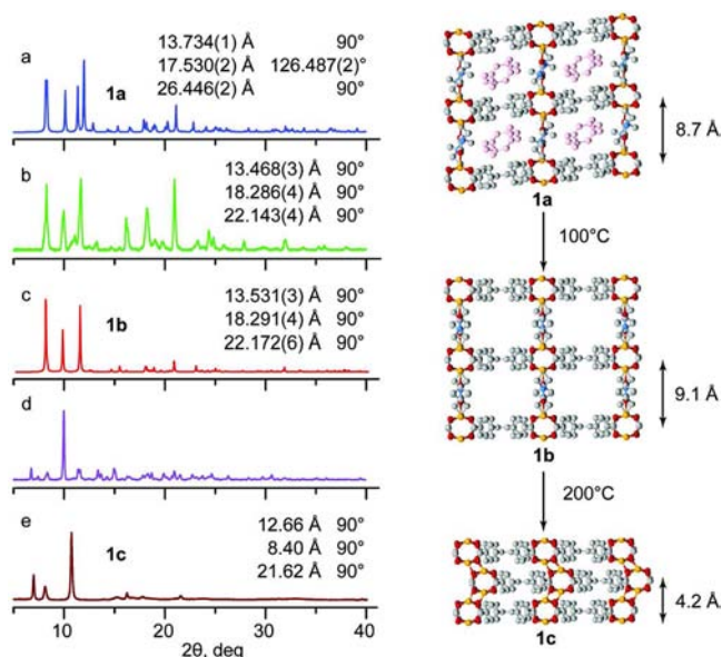
Figure 2. Temperature-dependent X-ray diffraction studies of 1. Left column: PXRD patterns of (a) 1a calculated from the X-ray crystal structure determined at 100 K, (b) 1a collected at room temperature, (c) 1b calculated from X-ray structure at 373 K, (d) the sample used in the ^2\text{H} NMR study, and (e) 1c. Right column: X-ray crystal structures of 1a collected at 100 K, 1b collected at 373 K, and the simulated structure of 1c based on the PXRD data. Golden, red, blue, and gray spheres represent Zn, O, N, and C atoms, respectively. Guest DEF molecules are shown in pink. H/D atoms have been removed for clarity.
